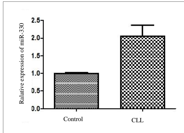
Fig. 2. Relative expression of miR-330 in two groups: CLL (n=30) and controls (n=30). Relative quantitation (RQ) for the miR-330 was significantly different in CLL and control ( p<0.001 ). Error bars show SE.
